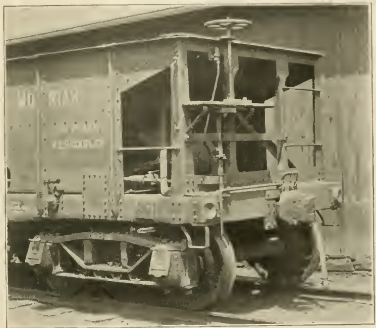
MORE EFFICIENT HAND BRAKE FOR LARGE CAPACITY CARS.
